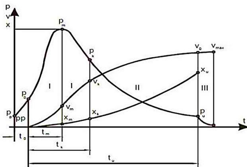
Fig. 1. Diagram of the change in propellant gas pressure - P , projectile velocity - V , and distance traveled - X as a function of time: t_0 - preliminary phase, t_k - first phase, t_u – time of the start of projectile movement to the projectile's exit from the barrel.
