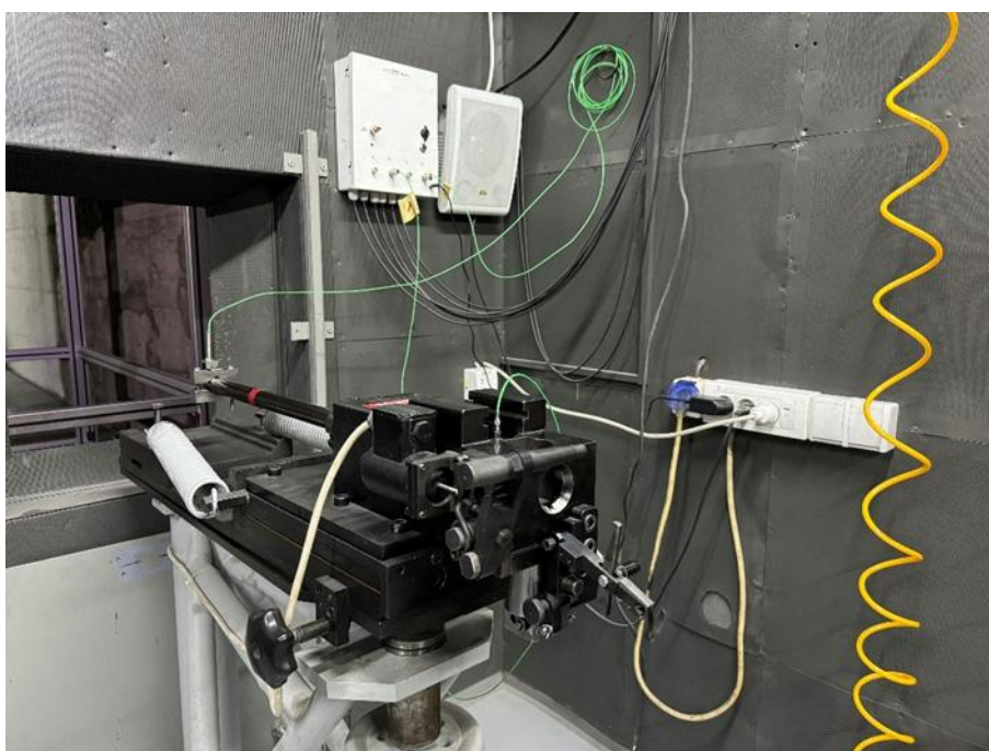
Fig. 4. Ballistic barrel holder for testing with measurement system
